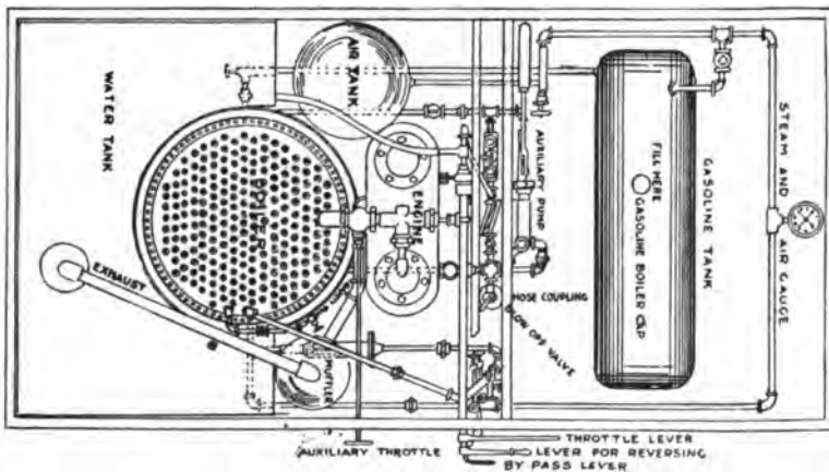
FIG. 247.—Plan Arrangement of the "Locomobile" Steam Carriage, showing position of the parts indicated in Fig. 245.
